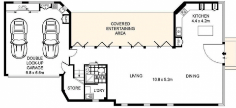
GROUND LEVEL
