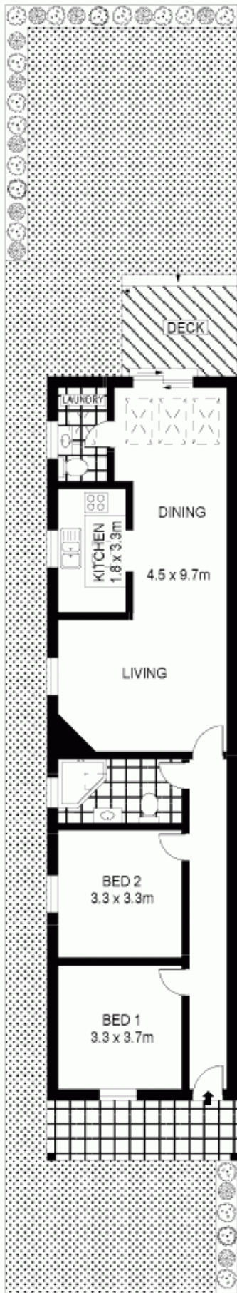
GROUND FLOOR
