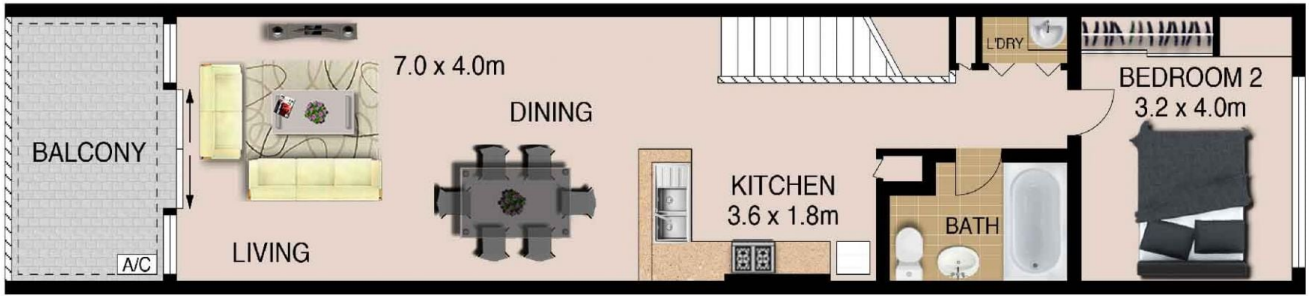
FIRST FLOOR
