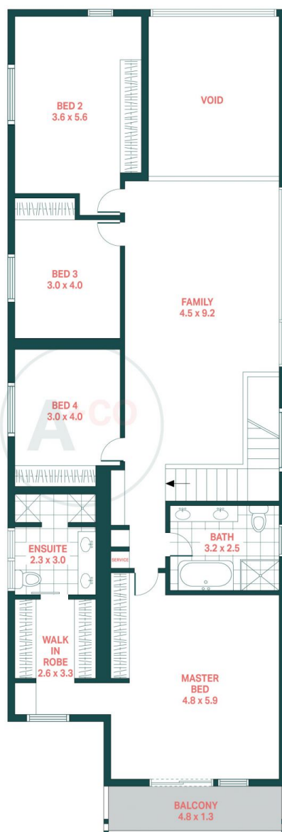
FIRST FLOOR
