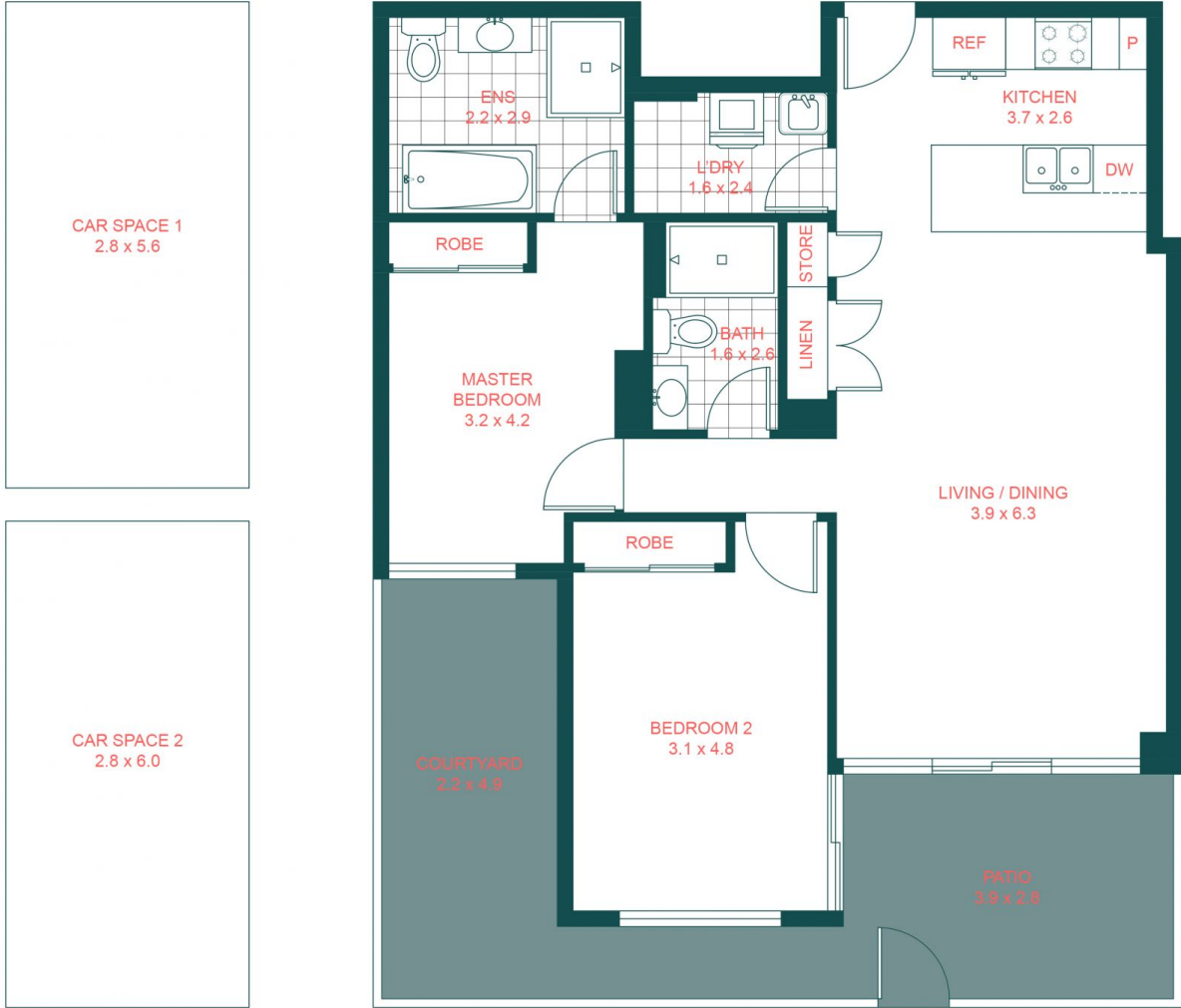
FLOOR PLAN
