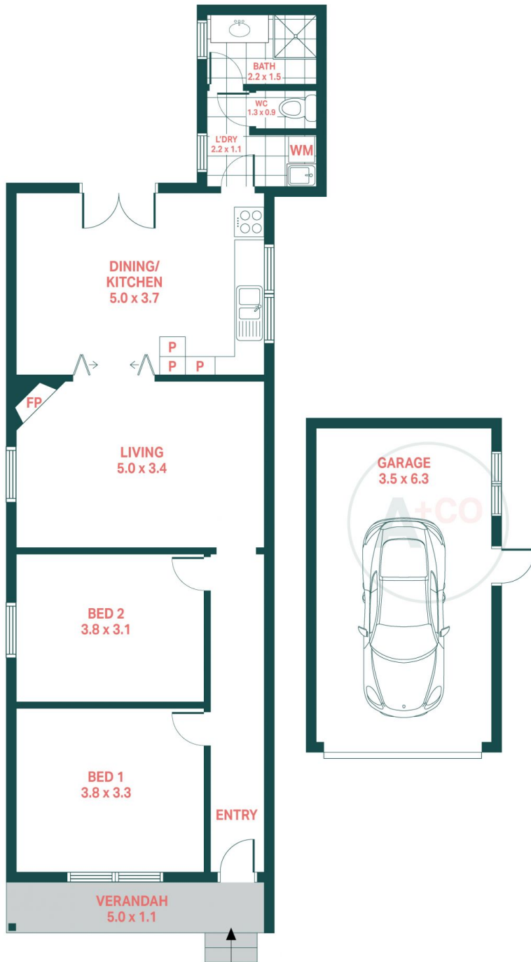
GROUND FLOOR
