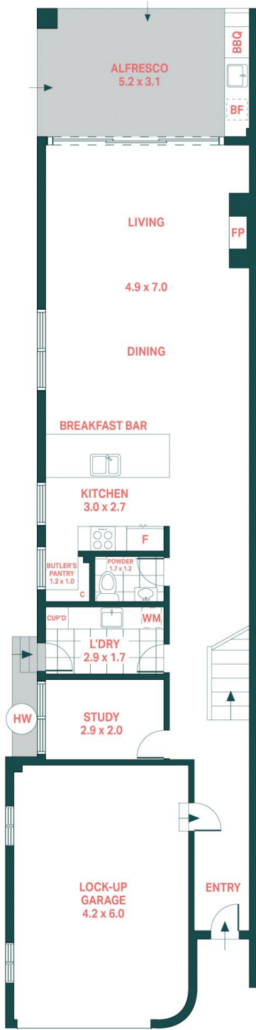
GROUND FLOOR
