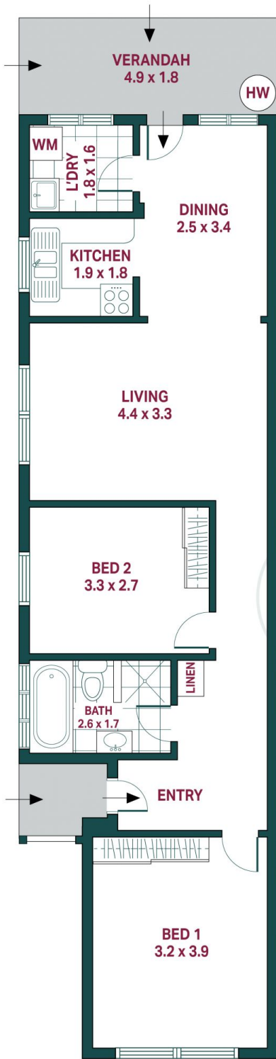
GROUND FLOOR
